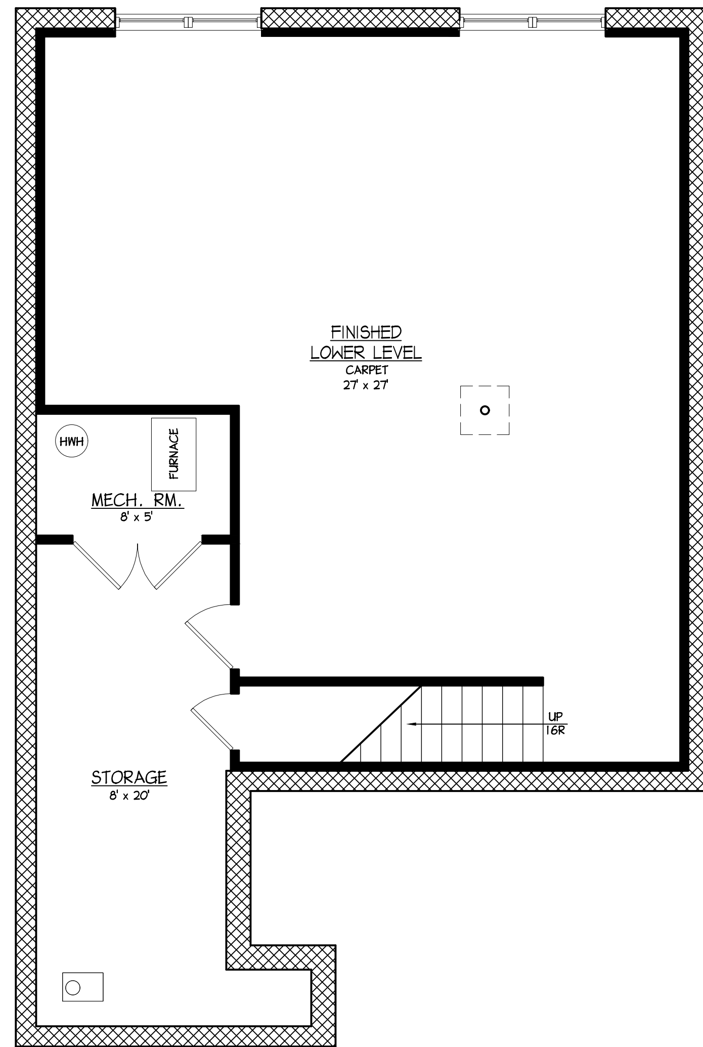
LOWER LEVEL PLAN
